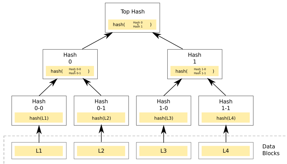
Figure 1: Merkle Tree - Wikipedia
