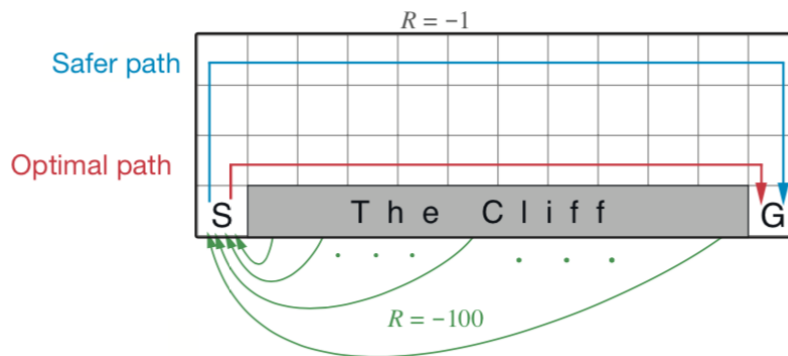
Figure 1: Cliff Walking
